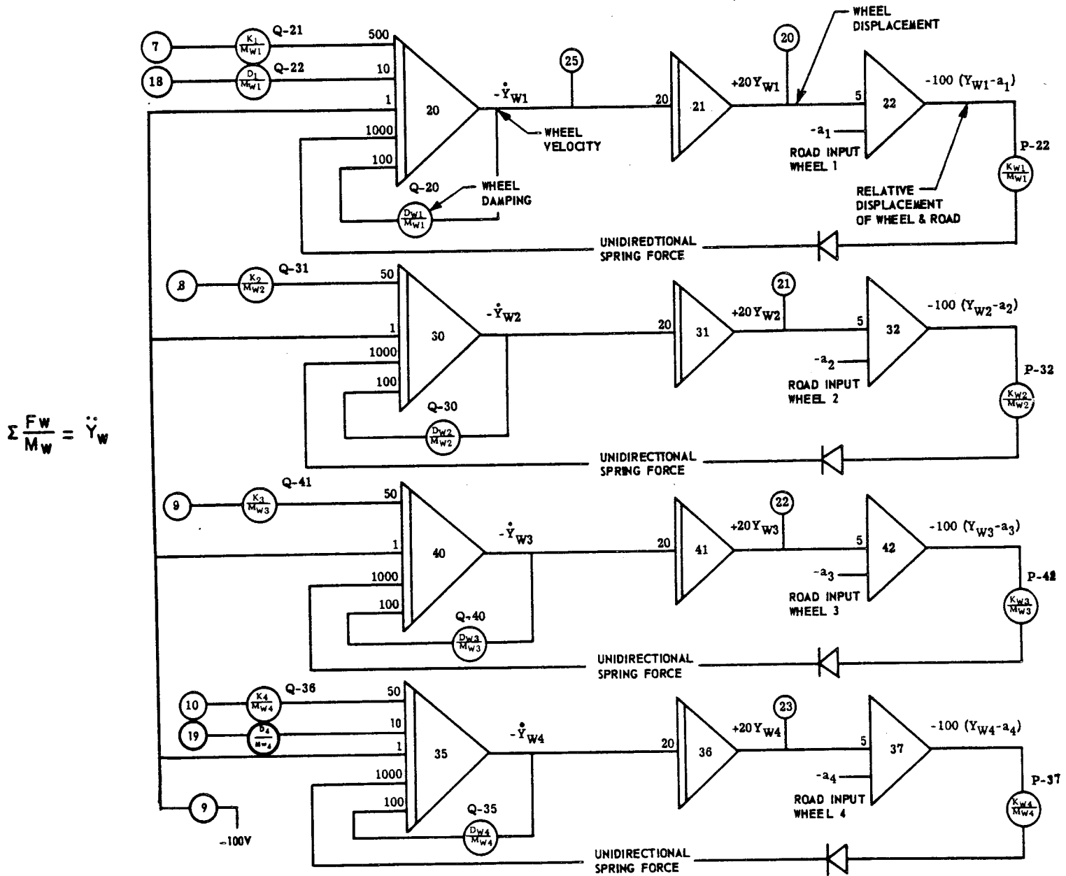
FIG. 11 WHEEL VELOCITY, AND DISPLACEMENT
