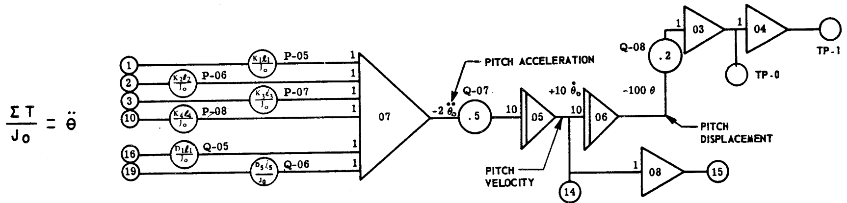
FIG. 13 C.G. PITCH ACCELERATION, VELOCITY, DISPLACEMENT
