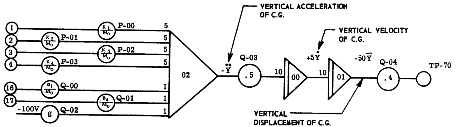
FIG. 12 C.G. VERTICAL ACCELERATION, VELOCITY, DISPLACEMENT
