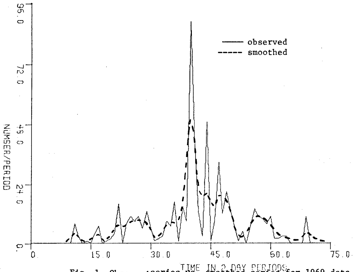
Fig. 1. Observed series vs. smoothed series for 1969 data.
