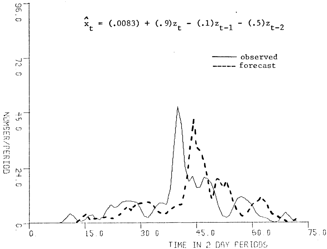
Fig. 4 Observed as 4-day ahead forecast series for 1969 smoothed data.
