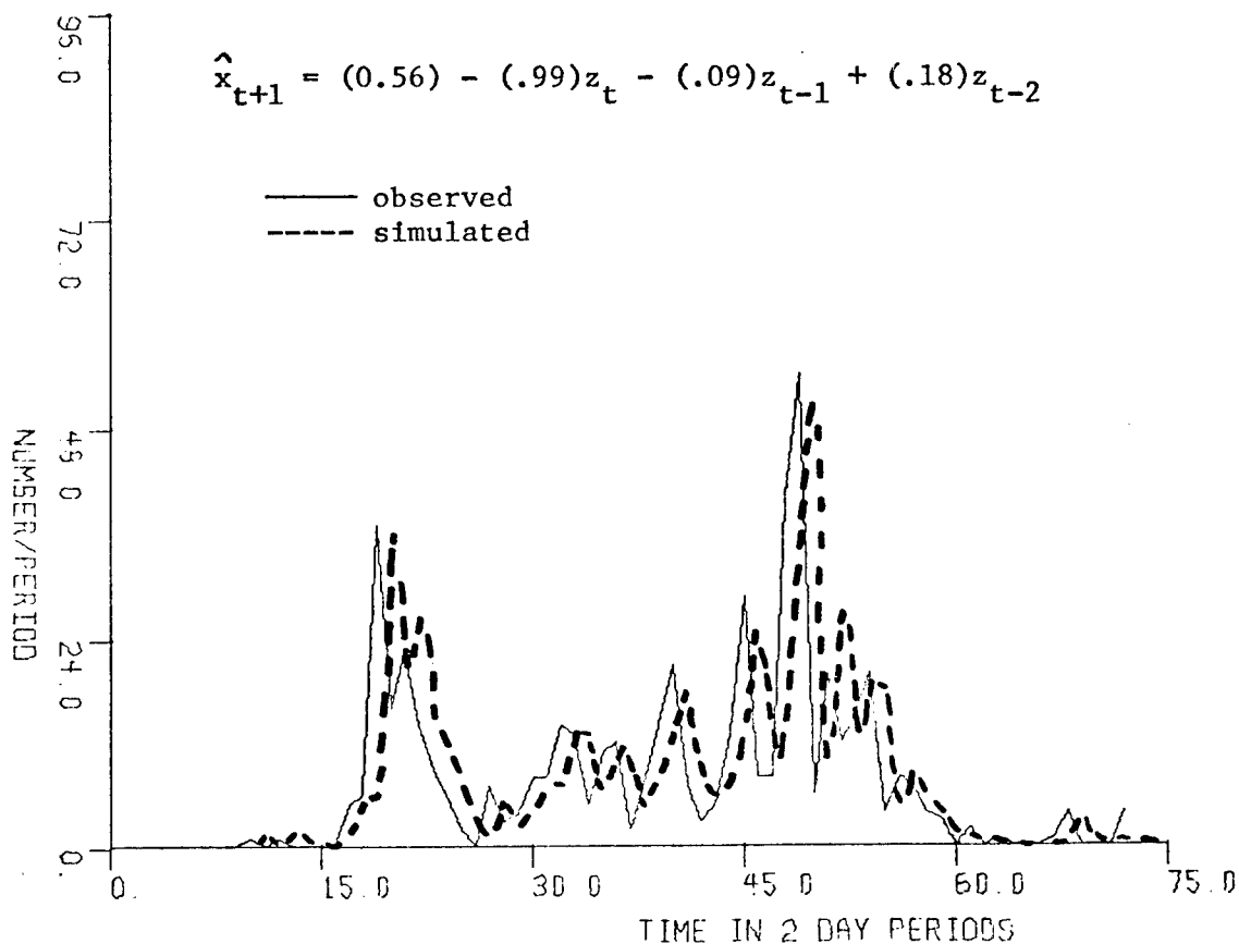
Fig. 10. Observed series vs. 1-day ahead forecast for 1971 raw density data. 540
