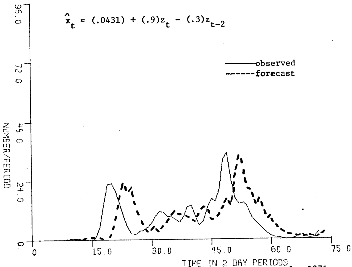
Fig. 6 Observed vs. 4-day ahead forecast series for 1971 smoothed data.
