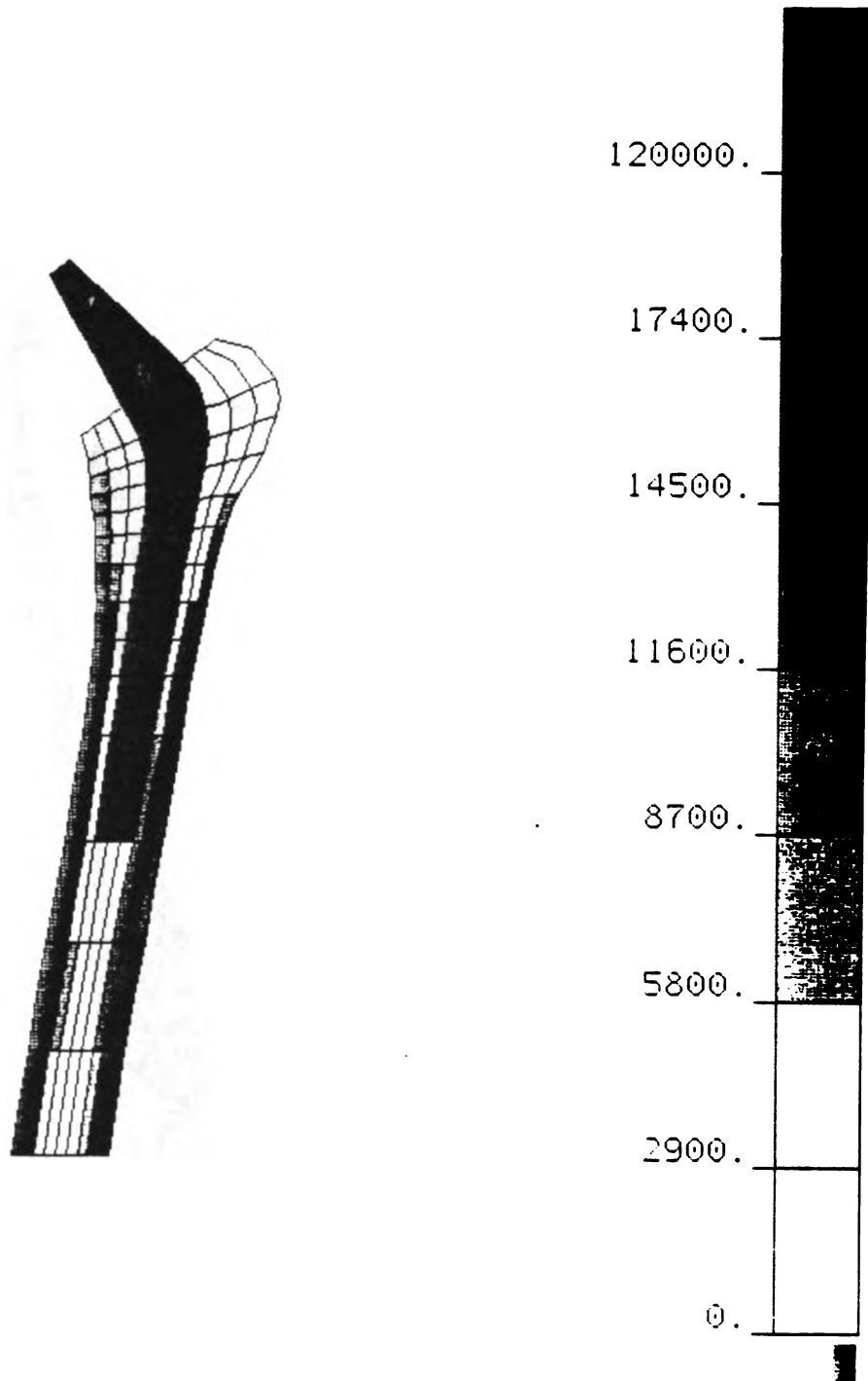
Figure 5: Distribution of the mean Young's modulus in the proximal femur
