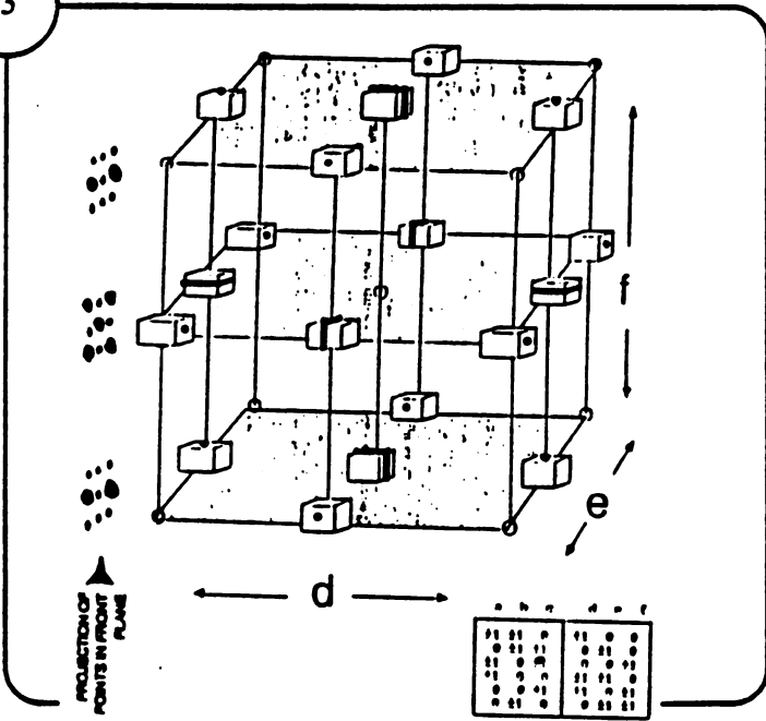
Box - Behnken 3^2 Fractional Design
