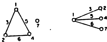
FIGURE 1. Linear Graphs for the 1_3 Orthogonal Array.
