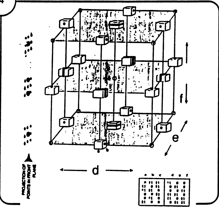
Bad - Barton 3^2 Fractional Design
