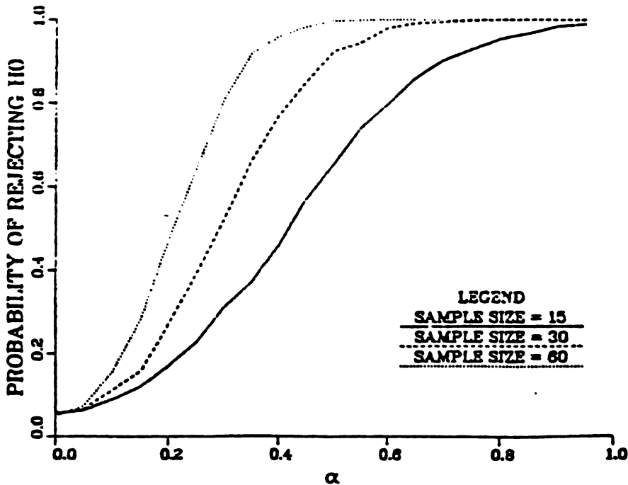
FIGURE 5: POWER OF 5%-LEVEL TEST H_0: F=G=LOGISTIC(0,1) VS. H_1: F=LOGISTIC(0,1), G=LOGISTIC(\alpha \neq 0,1)
